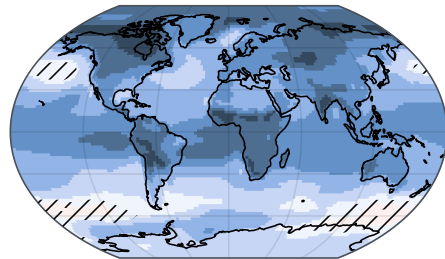
\Delta TREFHT due to clubb_C8
