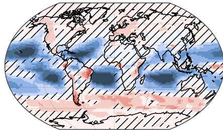
\Delta SWCF due to zmconv_tiedke_add
