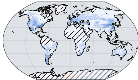
\Delta LHFLX due to d_max
