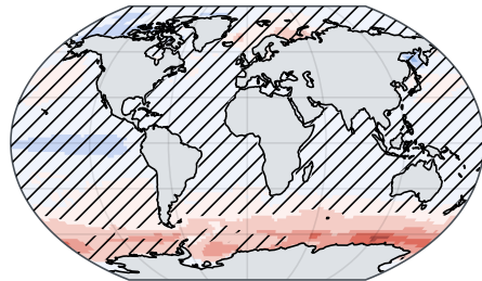
\Delta SST due to EGIDFQ
