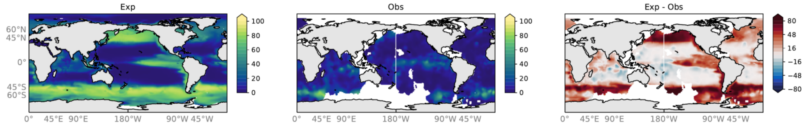
OMIP2-newspinup mean over years: 1680-1681 Observations: Seiter Opal(wt-%)
