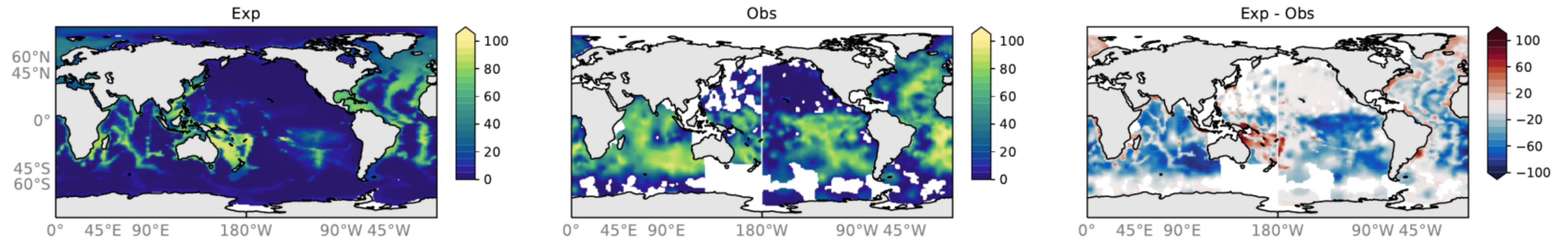
OMIP2-newspinup mean over years: 1680-1681 Observations: Seiter CaCO 3 (wt-%)
