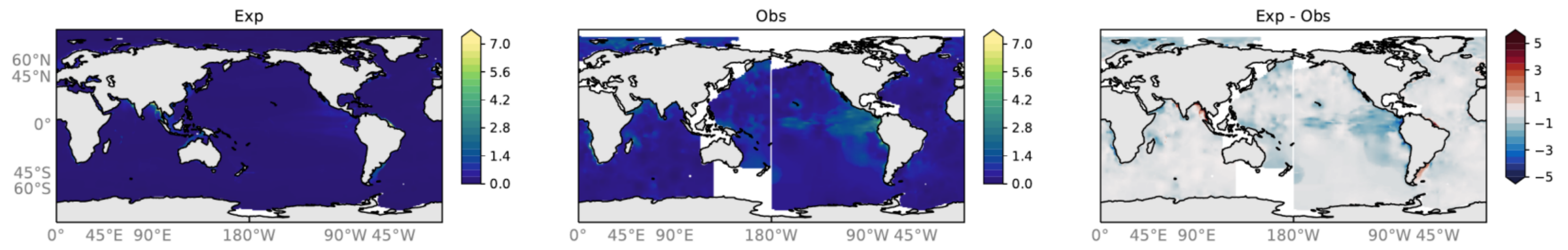
OMIP2-spinup mean over years: 1680-1681 Observations: Seiter TOC (wt-%)
