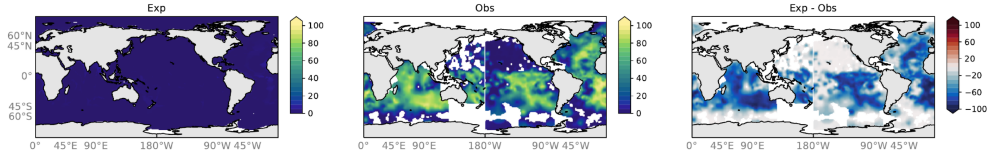
OMIP2-spinup mean over years: 1680-1681 Observations: Seiter CaCO 3 (wt-%)
