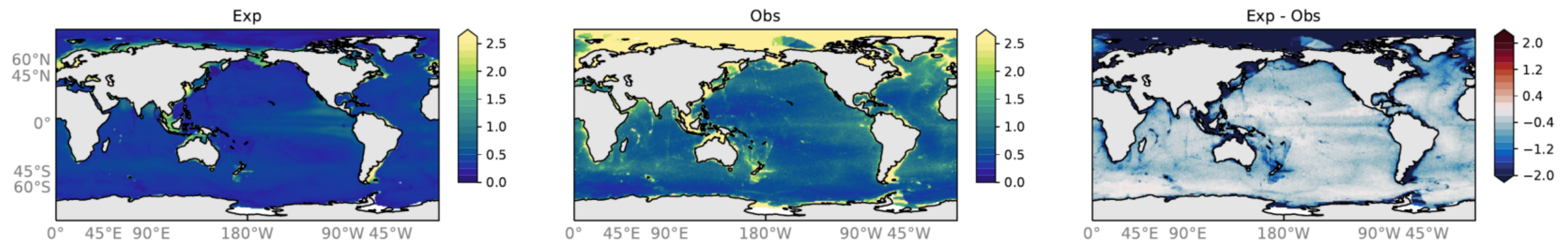
OMIP2-spinup mean over years: 1680-1681 Observations: Joergensen positive downward O 2 -flux (mmol O 2 m -2 d -1 )
