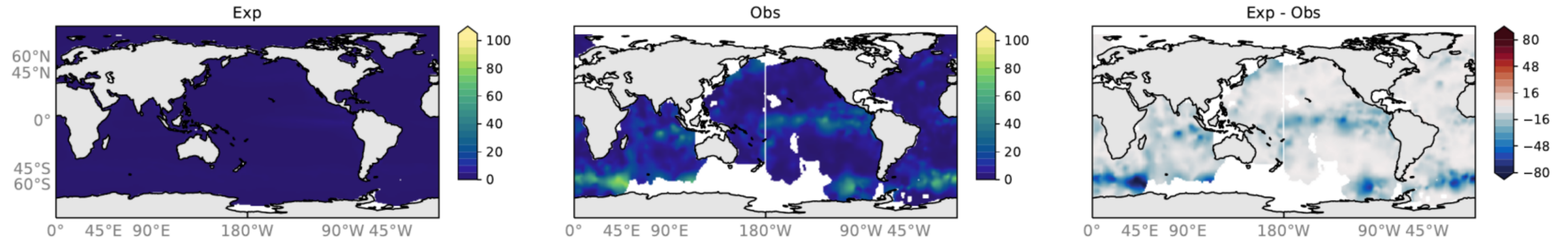
OMIP2-spinup mean over years: 1680-1681 Observations: Seiter Opal (wt-%)
