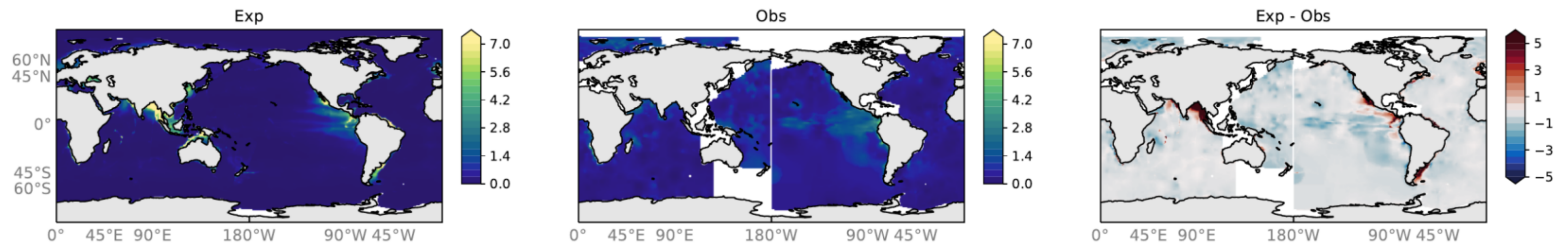
RYF6162 mean over years: 1770-1773 Observations: Seiter TOC (wt-%)
