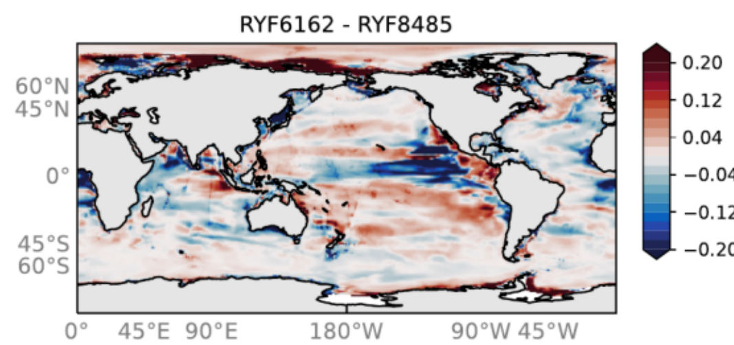
RYP6162 - RYP8485 Observations: Joergensen positive downward O 2 -flux (mmol O 2 m -2 d -1 )
