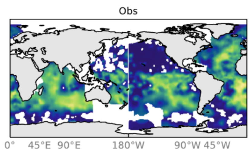
RYF8485 mean over years: 1770-1773 Observations: Seiter \text{CaCO}_3 (wt-%)
