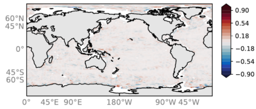
Transfer efficiency for Opal flux 100.0 → 1000.0 RYF6162 1770-1773 - RYF8485 1770-1773 -
