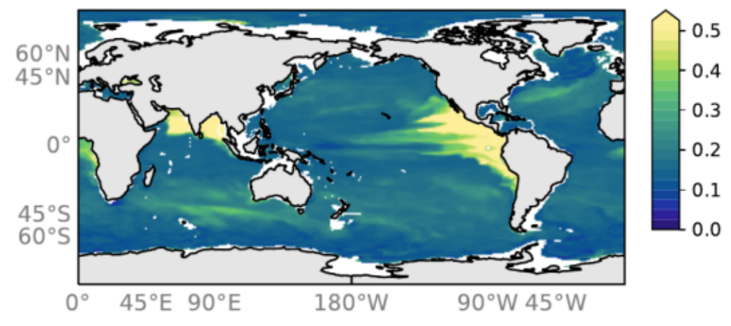
Transfer efficiency for POC flux 100.0 → 1000.0 RYF8485 1770-1773
