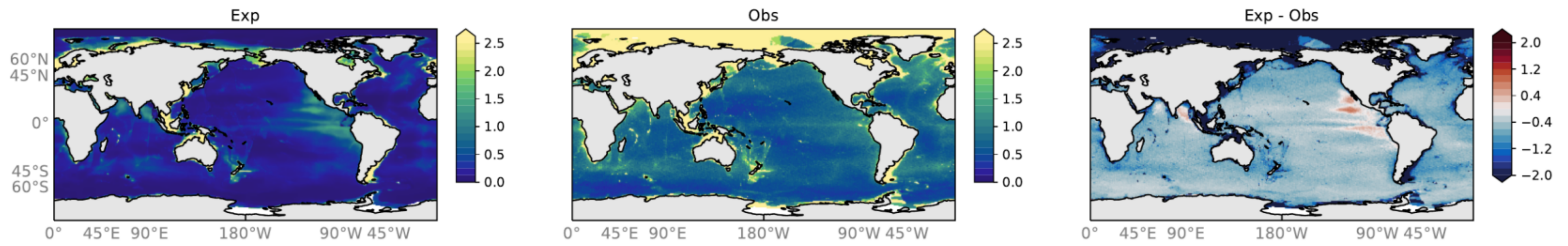
RYP6162 mean over years: 1770-1770 Observations: Joergensen positive downward O 2 -flux (mmol O 2 m -2 d -1 )
