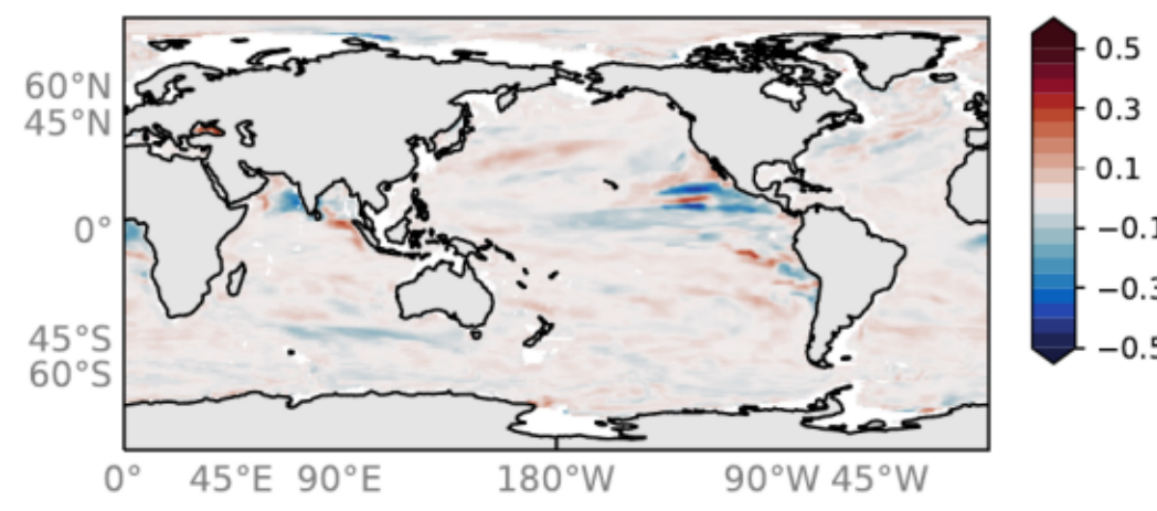
Transfer efficiency for POC flux 100.0 → 1000.0 RYF6162 1770-1773 - RYF8485 1770-1773 -
