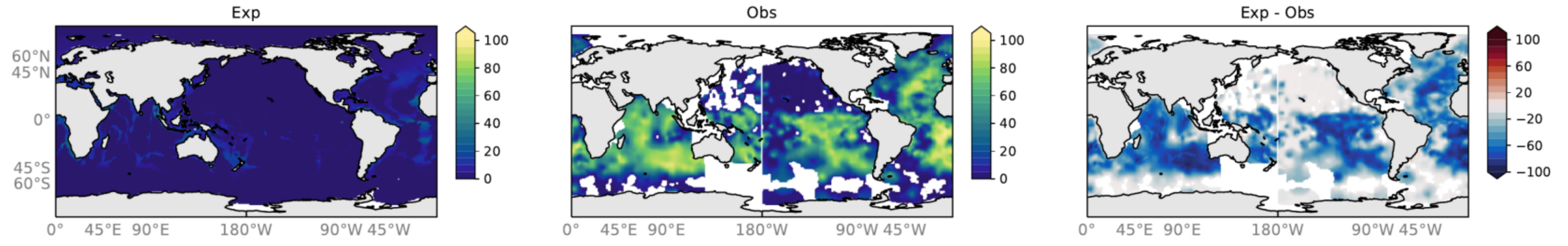
RYF6162 mean over years: 1770-1773 Observations: Seiter \text{CaCO}_3 (wt-%)
