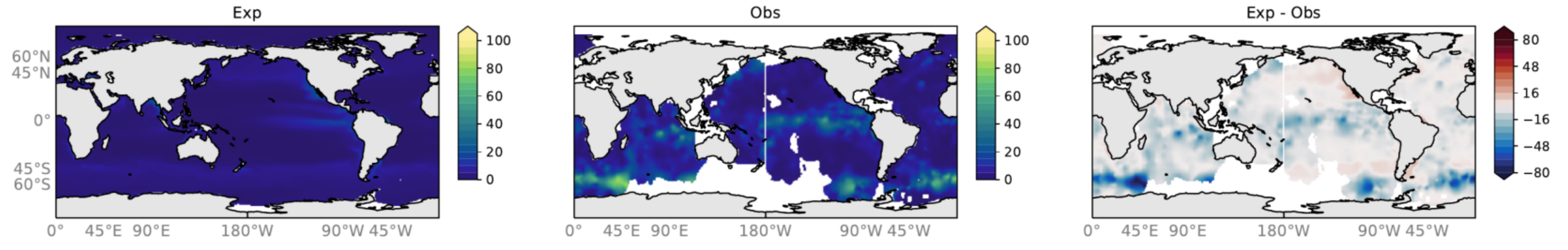
RYP6162 mean over years: 1770-1773 Observations: Seiter Opal(wt-%)
