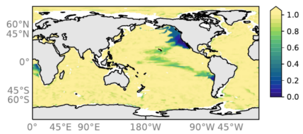
Transfer efficiency for CaCO 3 flux 100.0 → 1000.0 RYF6162 1770-1773
