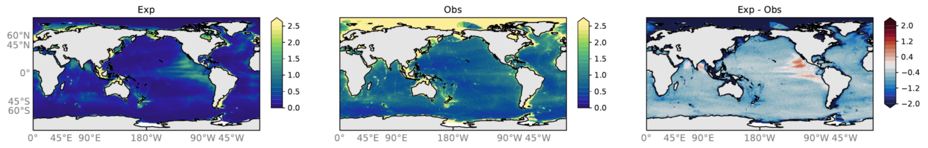
RYP8485 mean over years: 1770-1773 Observations: Joergensen positive downward O 2 -flux (mmol O 2 m -2 d -1 )
