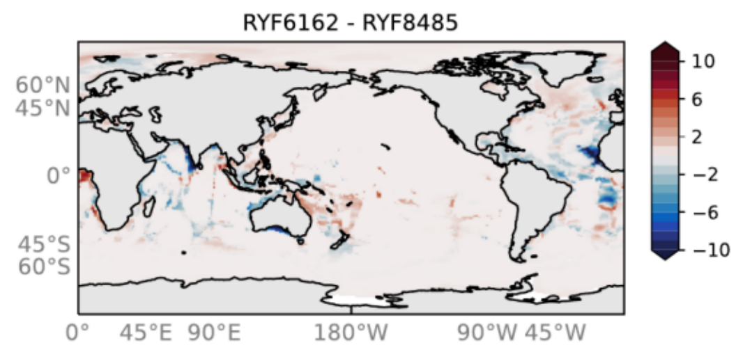
RYF6162 - RYF8485 \text{CaCO}_3 (wt-%)
