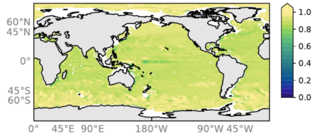
Transfer efficiency for Opal flux 100.0 → 1000.0 RYF6162 1770-1773
