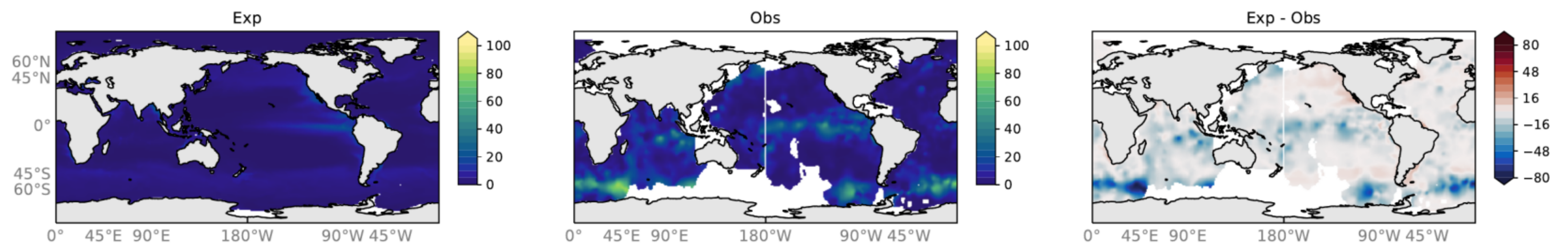
RYF8485 mean over years: 1770-1773 Observations: Seiter Opal (wt-%)
