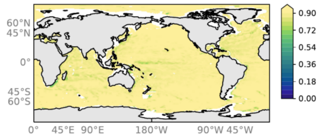
Transfer efficiency for Opal flux 100.0 → 1000.0 RYF8485 1770-1773
