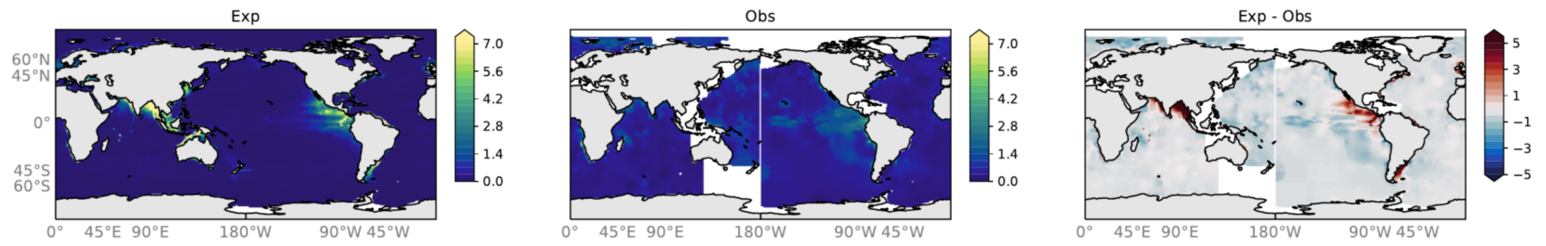
RYF8485 mean over years: 1770-1773 Observations: Seiter TOC (wt-%)
