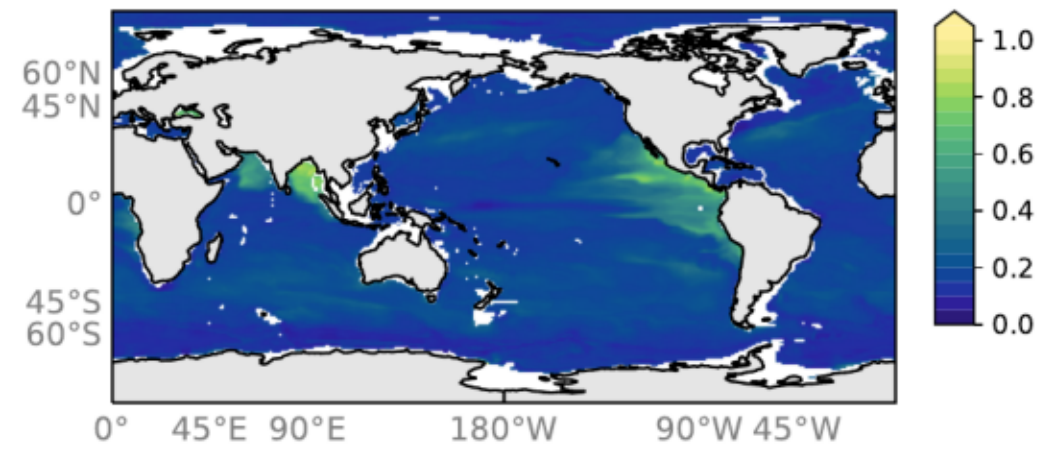
Transfer efficiency for POC flux 100.0 → 1000.0 RYF6162 1770-1773
