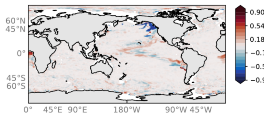
Transfer efficiency for CaCO 3 flux 100.0 → 1000.0 RYF6162 1770-1773 - RYF8485 1770-1773 -
