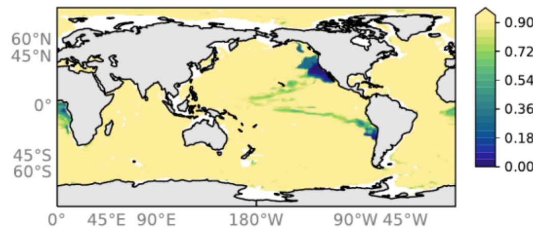
Transfer efficiency for CaCO 3 flux 100.0 → 1000.0 RYF8485 1770-1773
